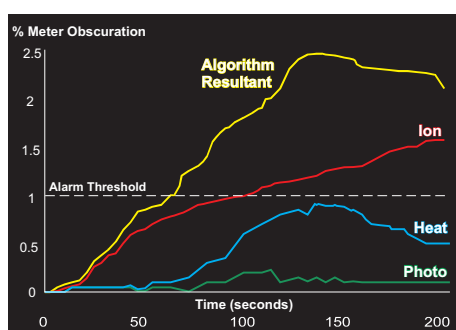
The example above demonstrates how the combined output from three sensors (re-sultant) reaches the alarm threshold earlier than any of the single sensors.
